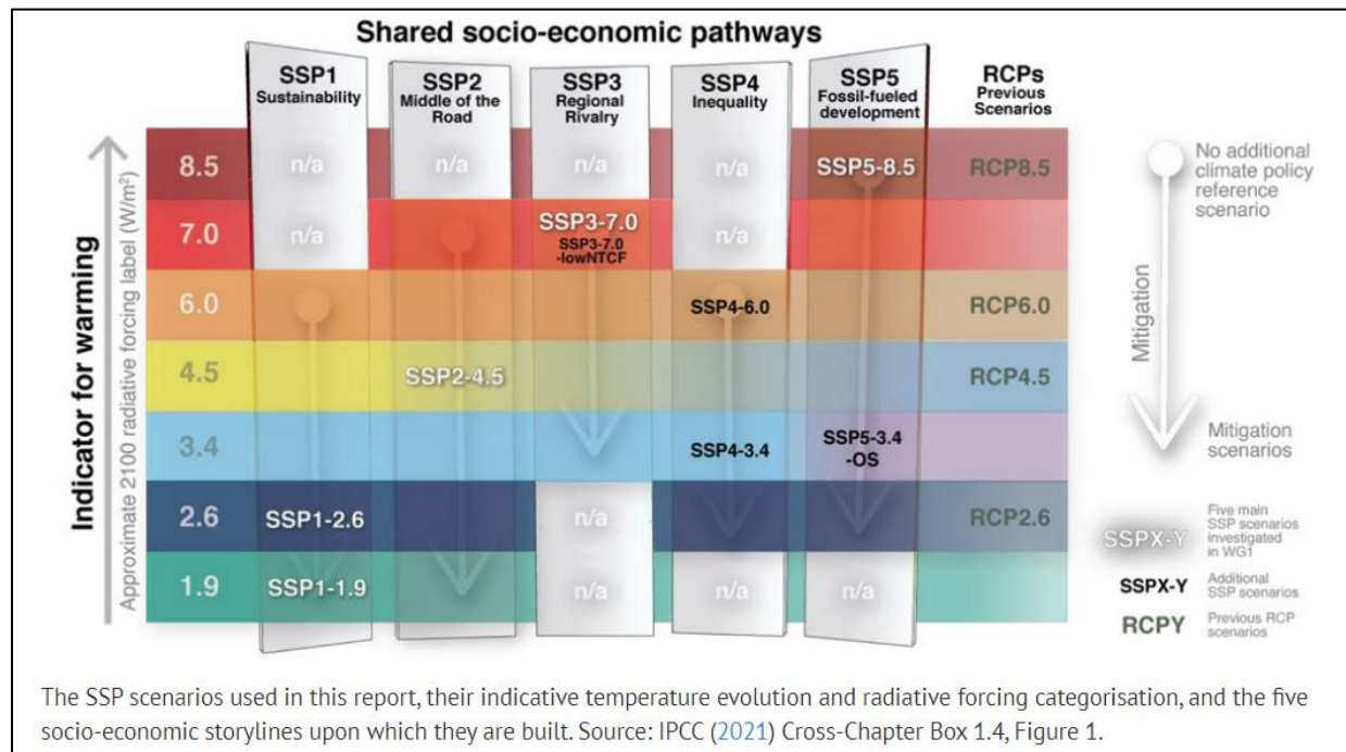
Figure 1. IPCC AR6 shared socio-economic pathways (IPCC, 2021)
