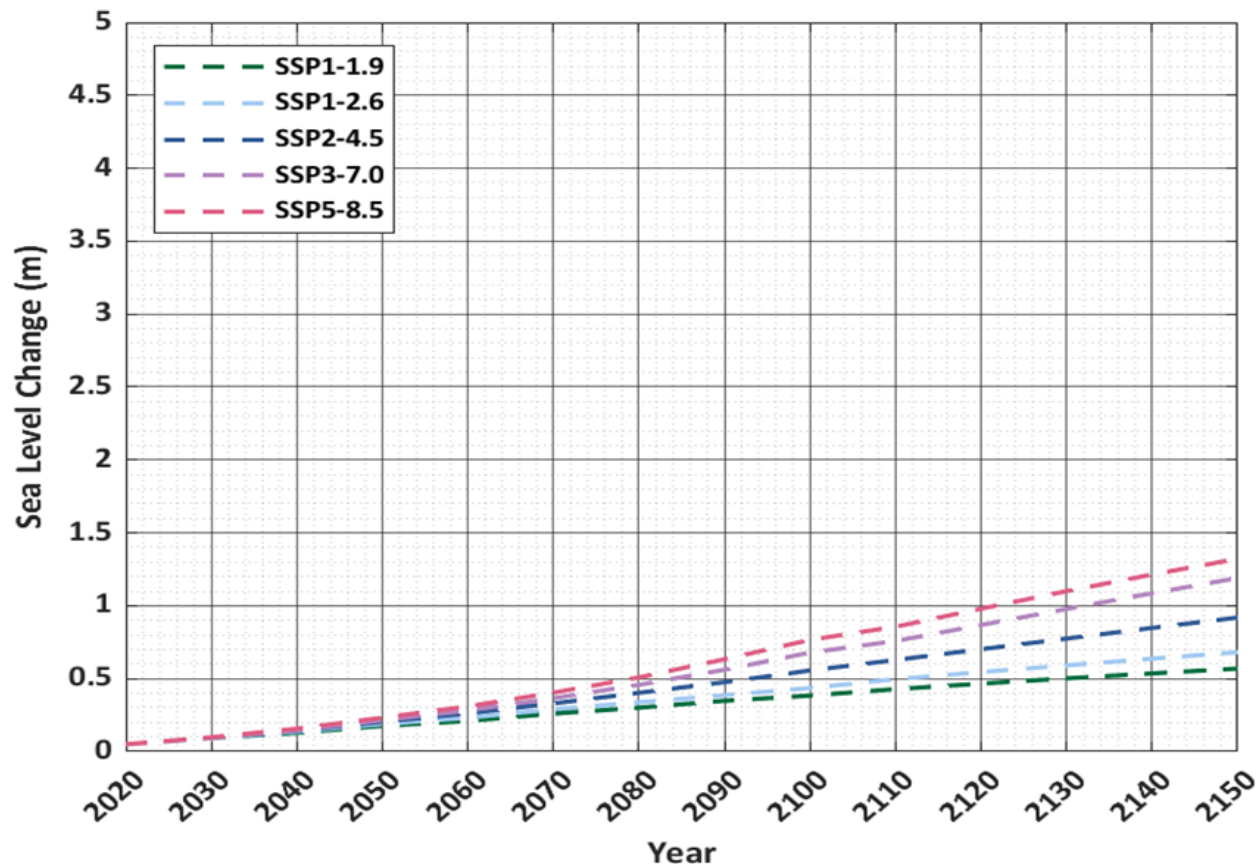
Figure 3. IPCC AR6 global sea level rise projections, 2020 to 2150 (IPCC, 2021)
