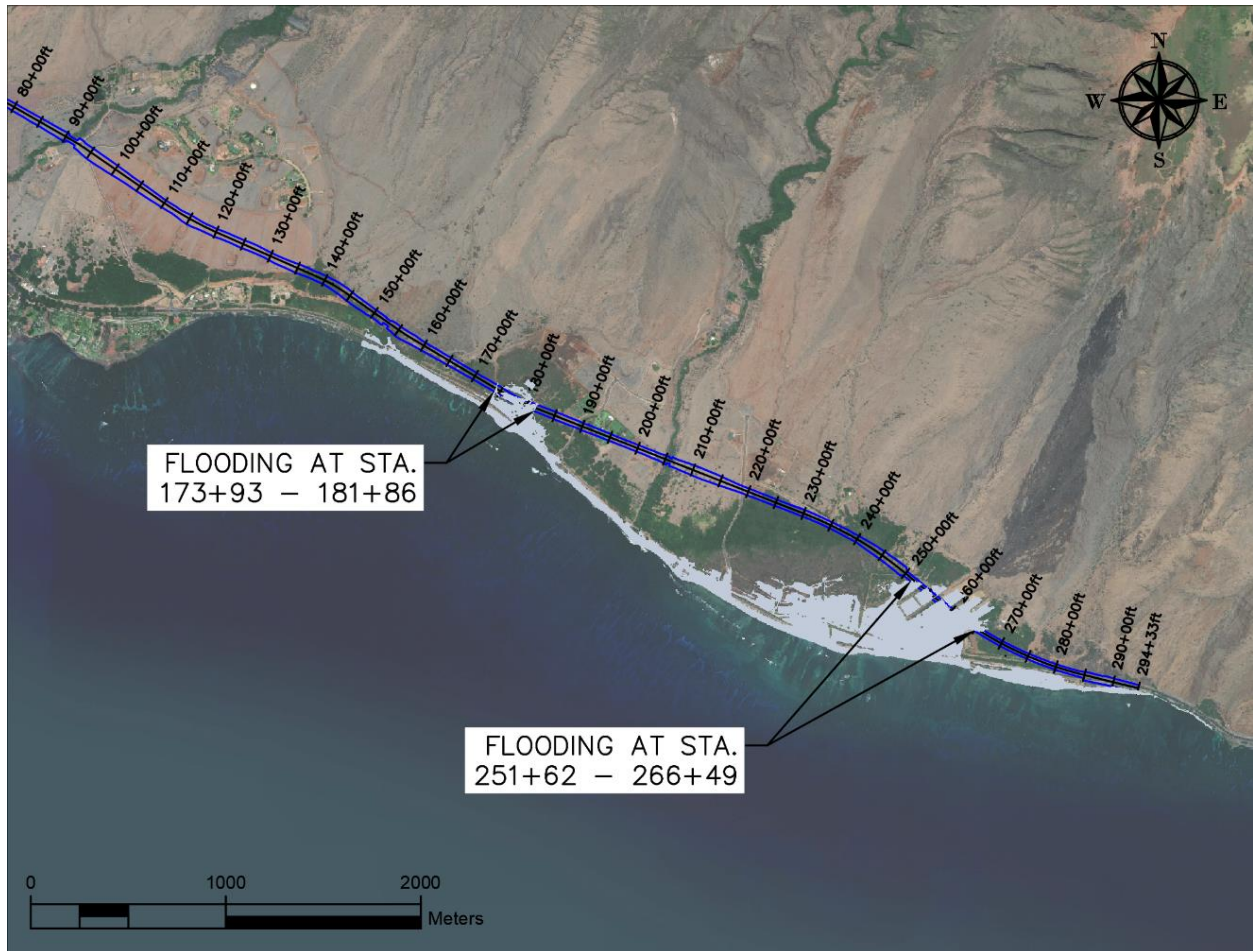
Figure 5-12. XBeach-NH modeled maximum flood extent (gray) for existing ground relative to alternative 4 (blue) alignment in the Ukumehame region.
