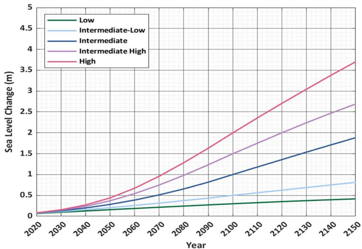
Figure 4. Task Force global sea level rise projections, 2020 to 2150 (Sweet, et al., 2022)
