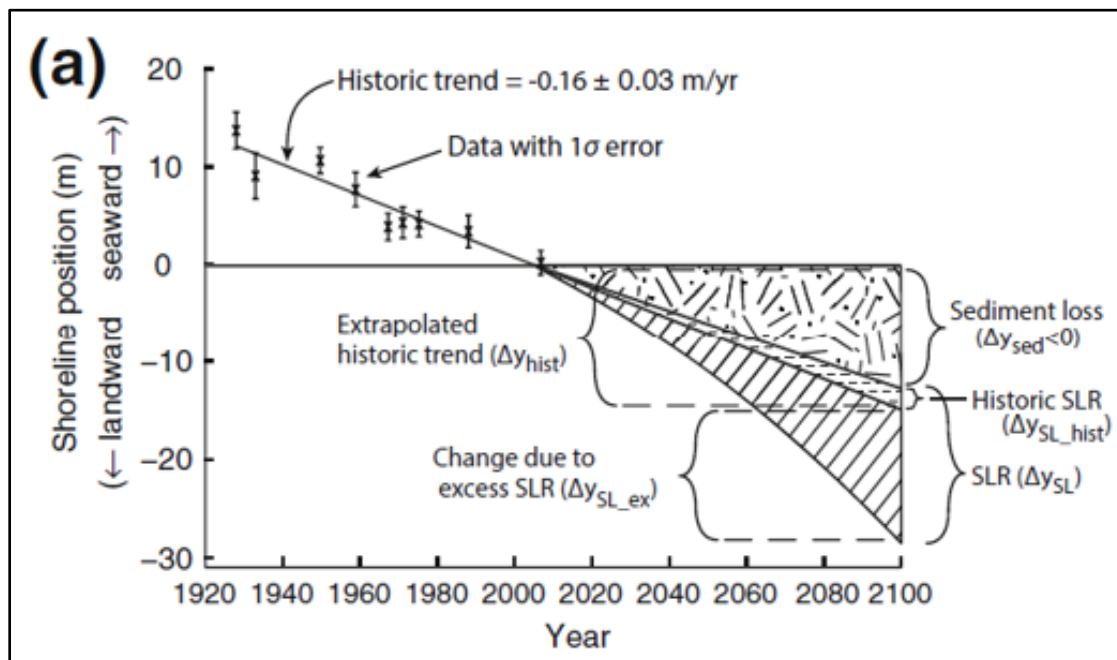
Figure 3-4. Graphic representation of the erosion model components from Anderson, et al., 2015
